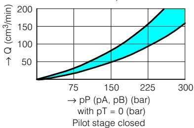
Leakage P→P1
