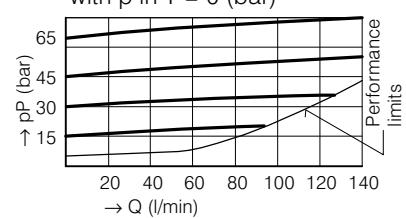
SDVB-3-..AR / ZR-10-..L p-Q characteristics with p in T = 0 (bar)
