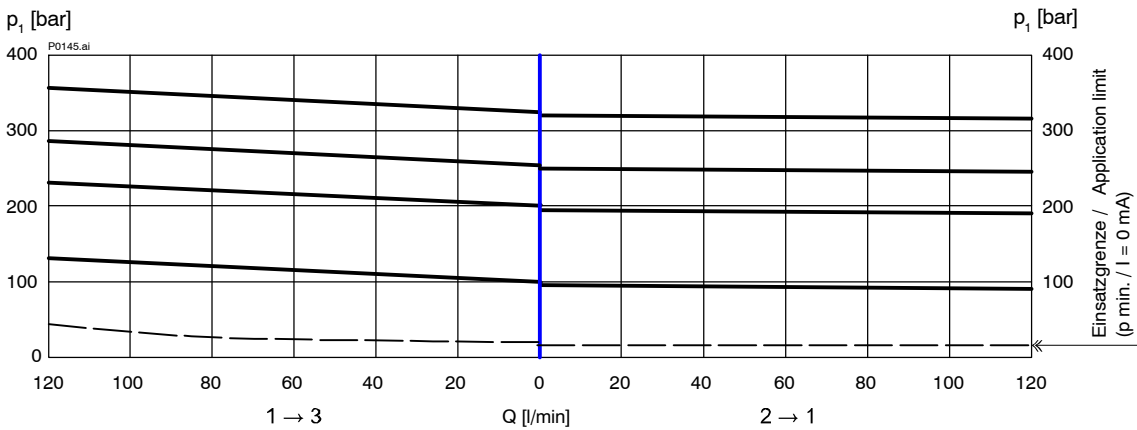
p = f(Q) Pressure - Flow rate characteristic [ p_N = 350 \text{ bar} ]
