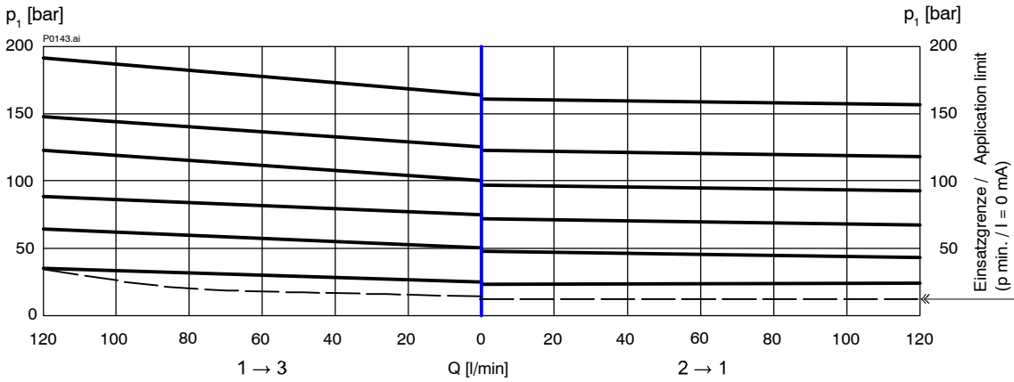
p = f(Q) Pressure - Flow rate characteristic [ p_N = 160 \text{ bar} ]
